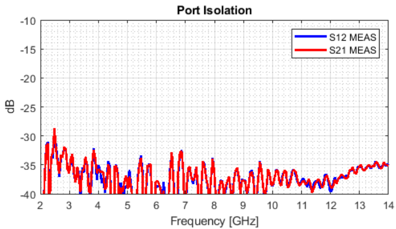
Fig 3.2. Measured port isolation.
