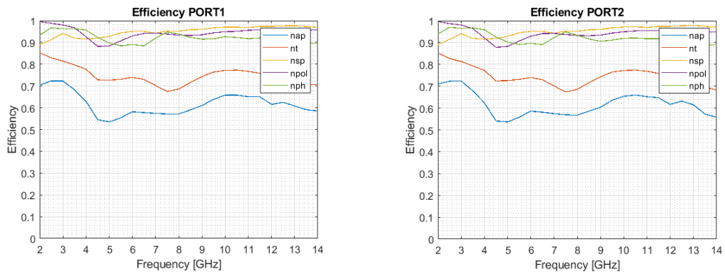
Fig 4.1. Estimated aperture efficiency of QRFH for each port.
