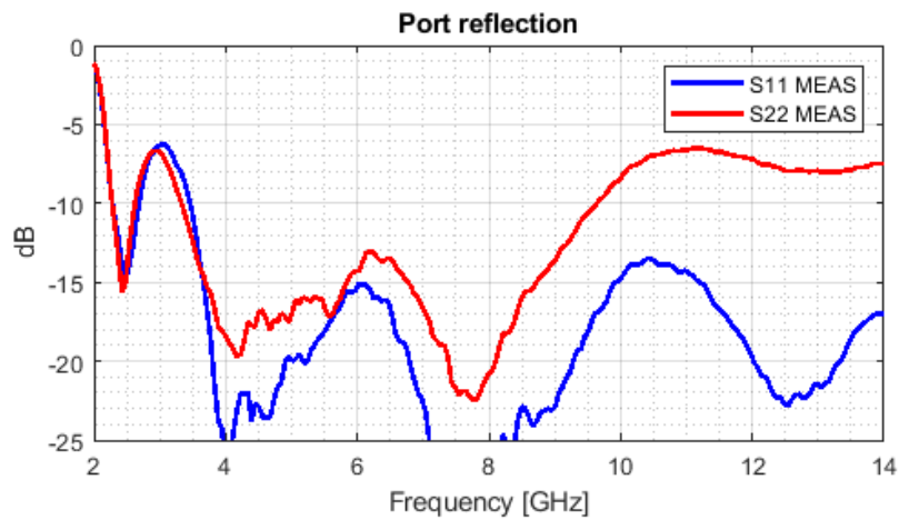
Fig 3.1. Measured port reflection
