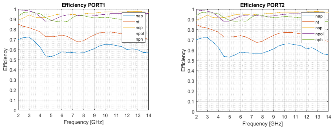
Fig 4.2. Estimated subefficiencies of QRFH for each port.
