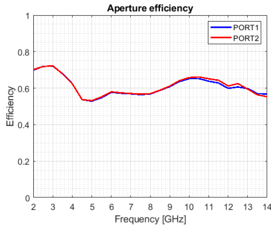
Fig 4.1. Estimated aperture efficiency of QRFH for each port.
