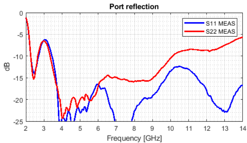
Fig 3.1. Measured port reflection
