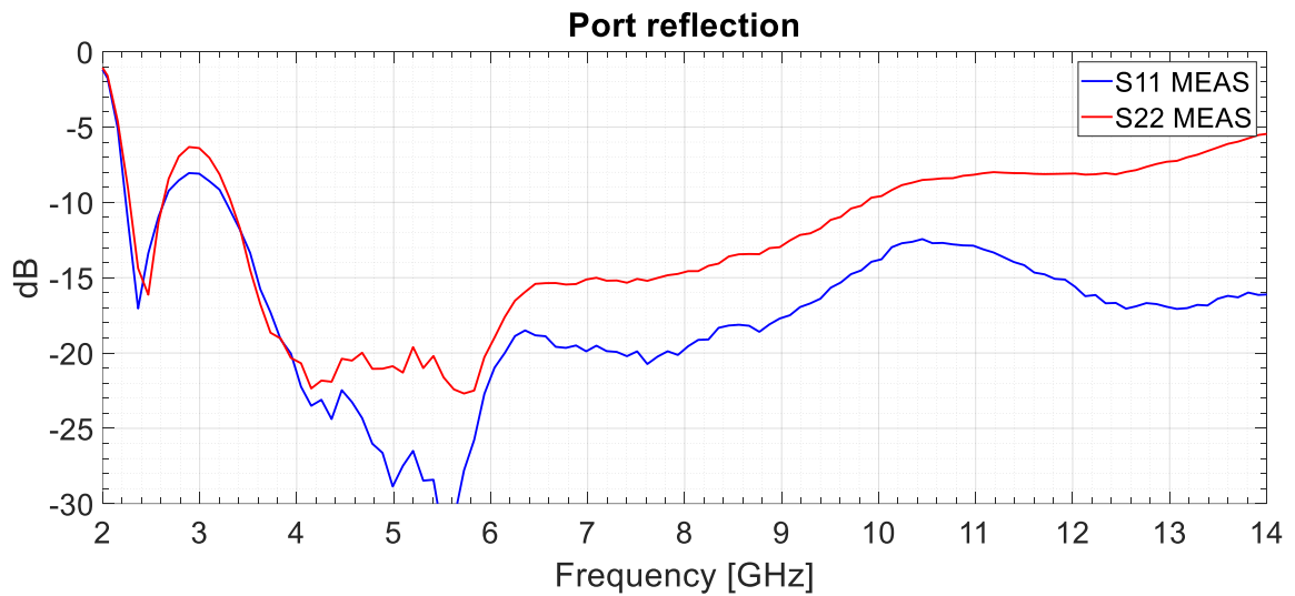
Fig 3.1. Measured port reflection
