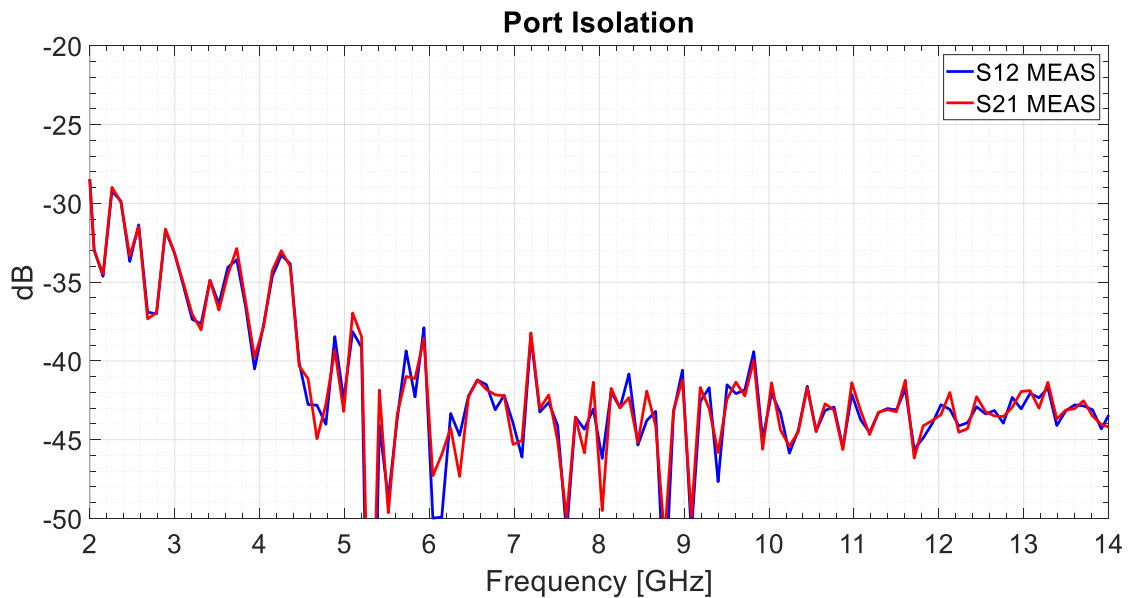
Fig 3.2. Measured port isolation.
