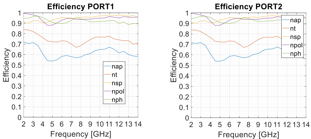
Fig 4.2. Estimated subefficiencies of QRFH for each port.
