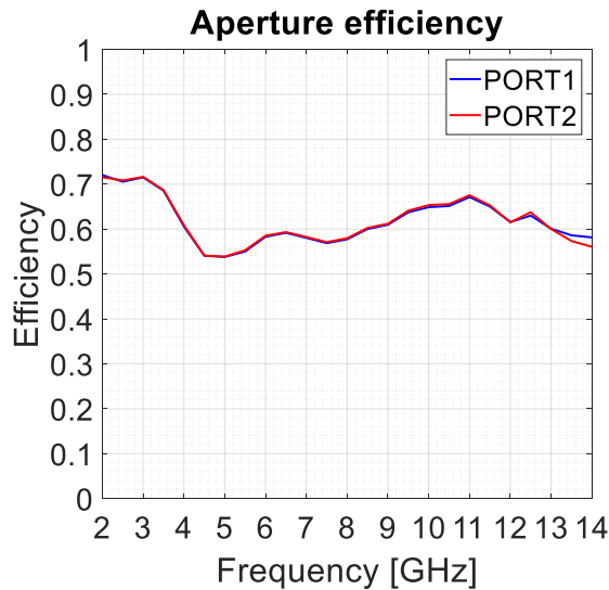
Fig 4.1. Estimated aperture efficiency of QRFH for each port.
